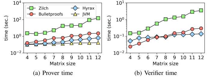
Fig. 11: Comparison between Zilch, Hyrax and Bulletproofs \mathcal{P} and \mathcal{V} timings (seconds) for the matrix multiplication benchmark, as well as the native JVM baseline execution (i.e., without generating a proof).
